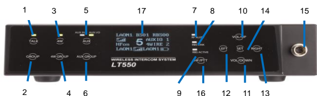
Front panel of the Base Station, LTWI-BS550
