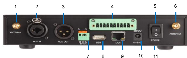
Rear panel of the Base Station, LTWI-BS550
